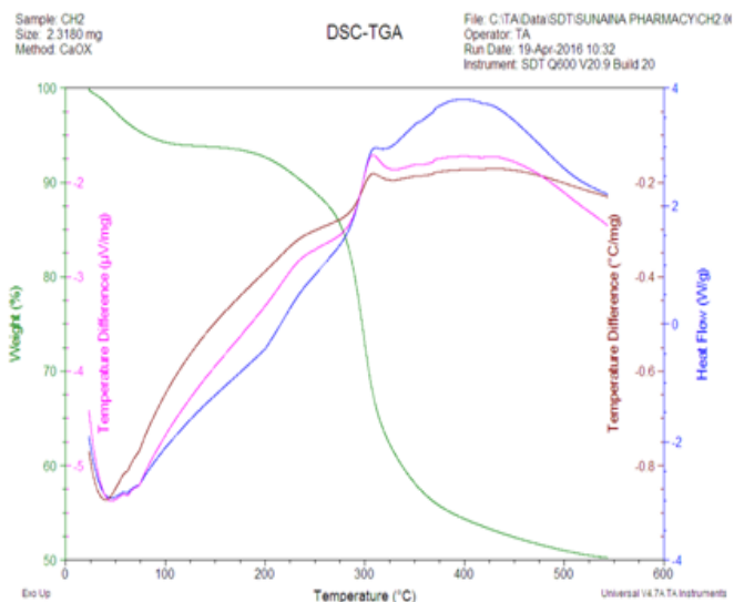
Figure 3. DSC-TGA thermogram of chitosan
