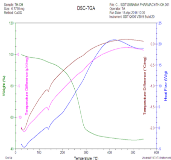
Figure 4. DSC-TGA thermogram of TCH
