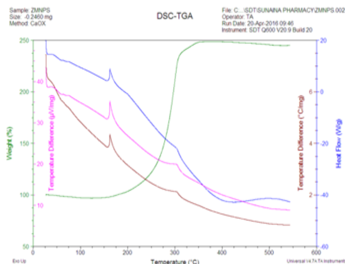
Figure 5. DSC-TGA thermogram of ZM-TCH-NPs
