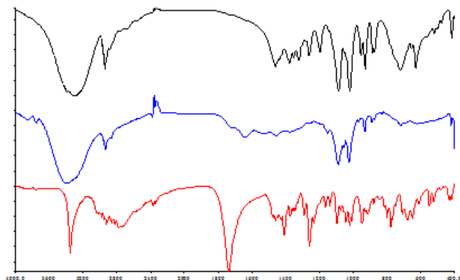
Figure 2. FTIR spectra of Zomitriptan (Lowest red), TCH (Middle Blue) and ZM-TCH-NPs (Highest Black).
